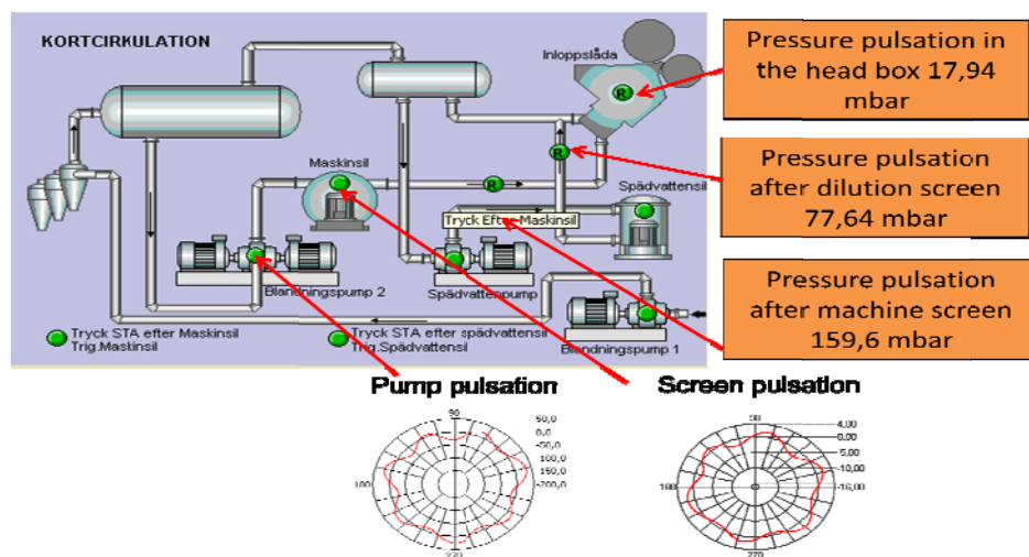
Figure 7: The origins of wet end pulsations are determined by the integrated monitoring of the DCS system
