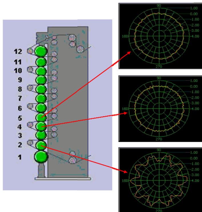
Figure 8: Synchronous time averaging (STA) analysis determines which roll in a supercalender is causing a barring problem.
