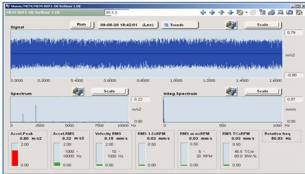
Figure 2: When a vibration alarm is acknowledged and activated by a mouse click on the combined process display, a pop-up window reveals the details of the vibration patterns in the process element.
