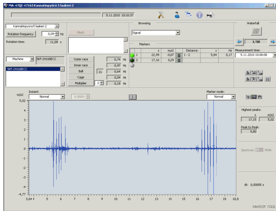
Figure 6: A signal sample from a troublesome support roller bearing housing vibration.
